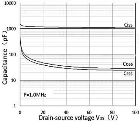
Figure 7. Capacitance Characteristics
