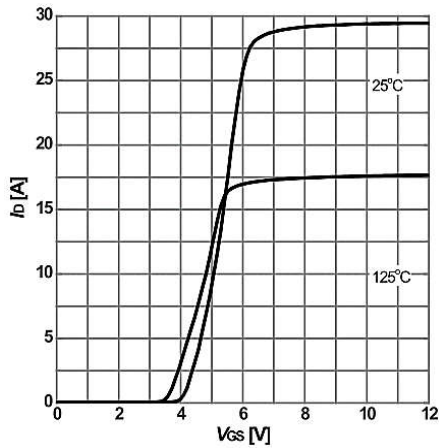
Figure 11: Type. transfer characteristics I_D=f(V_{GS}); V_{DS}=20\text{V}; parameter: T_J
