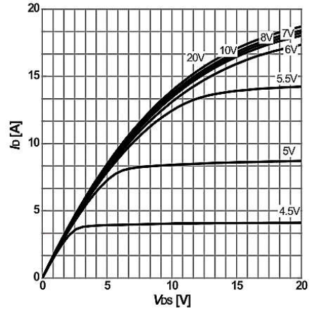
Figure 8: Typ. output characteristics I_D=f(V_{DS}); T_J=125^{\circ}\text{C}; parameter: V_{GS}
