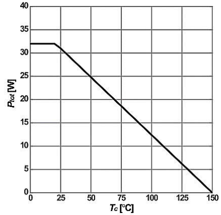
Figure2: Power dissipation (FullPAK)
