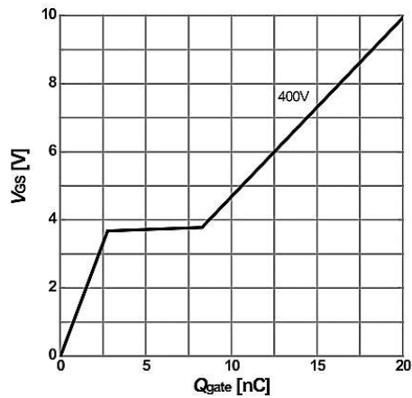
Figure 12: Type. gate charge V_{GS}=f(Q_{gate}); I_D=3.2\text{A pulsed}; V_{DS}=480\text{V}
