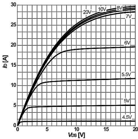
Figure 7: Typ. output characteristics I_D=f(V_{DS}); T_J=25^{\circ}\text{C}; parameter: V_{GS}
