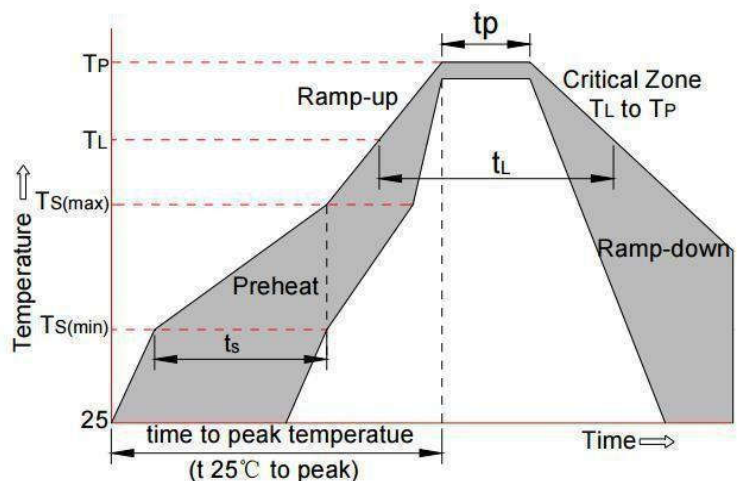
FIG.2: Reflow condition
