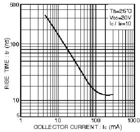
Fig.6 Rise time vs. collector current
