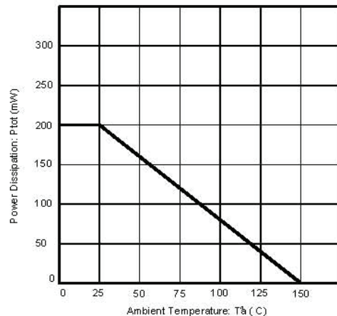
Fig.10 Power Dissipation vs Ambient Temperature
