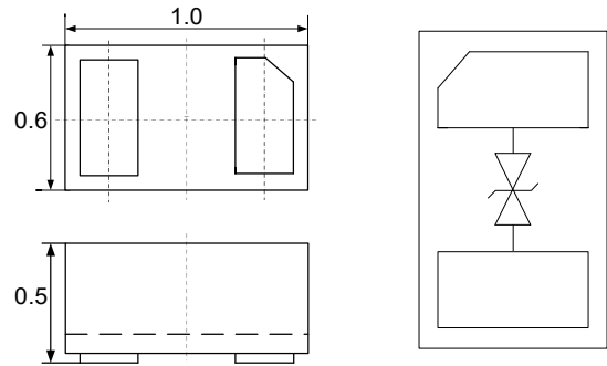
Package Dimensions
