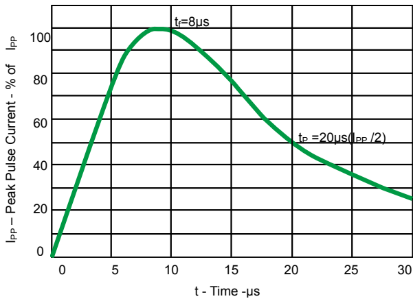
Fig 1. Pulse Waveform
