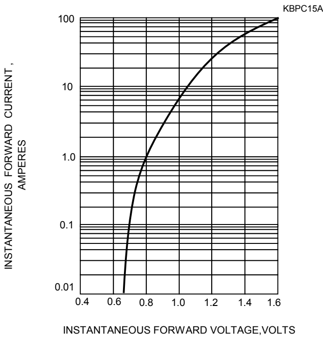
FIG.3-TYPICAL FORWARD CHARACTERISTICS
