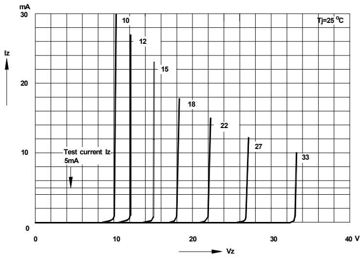
Breakdown characteristics T J = constant (pulsed)
