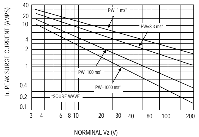
Fig.2 Maximum Non-Repetitive Surg Current versus Nominal Vz (V)
