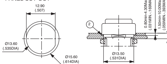
② - O-ring
