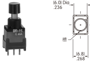
BB15AP-FA
