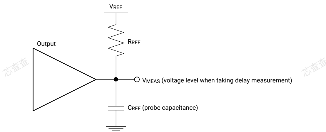
Figure 1: Single-Ended Test Setup
