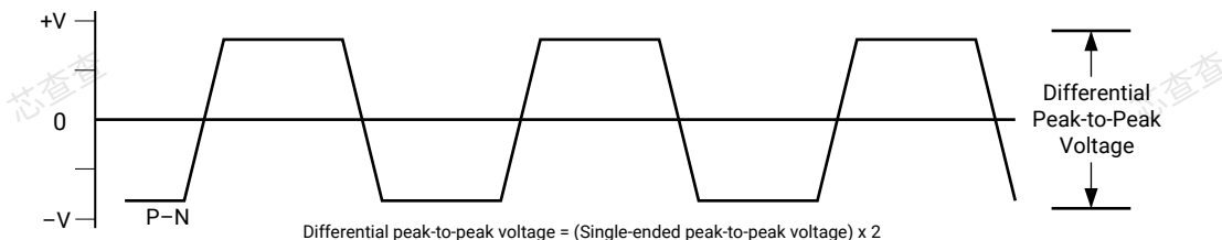
Figure 4: Differential Peak-to-Peak Voltage
