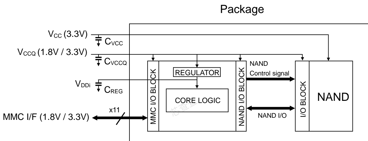
Figure 1 THGBMJG6C1LBAB7 Block Diagram
